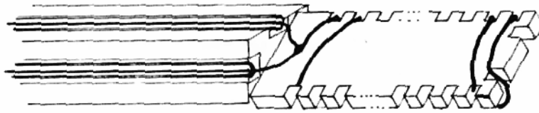
CONTINUOUS CAPILLARIES CONTAINING LEAD WIRES
